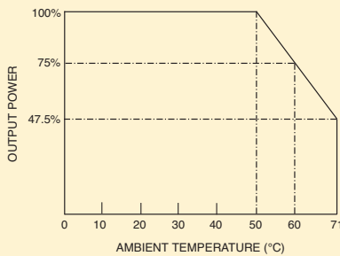
FIGURE 5 HSP Output Power vs. Ambient Temperature
