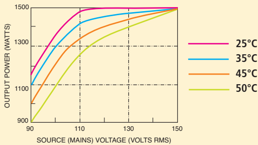
FIGURE 6 HSP 1500W Output Power vs. Source Voltage for Various Ambient Temperatures
